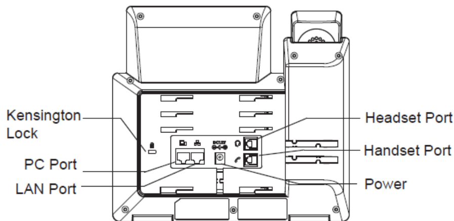
Figure 4: GRP2600 Back / Side View
