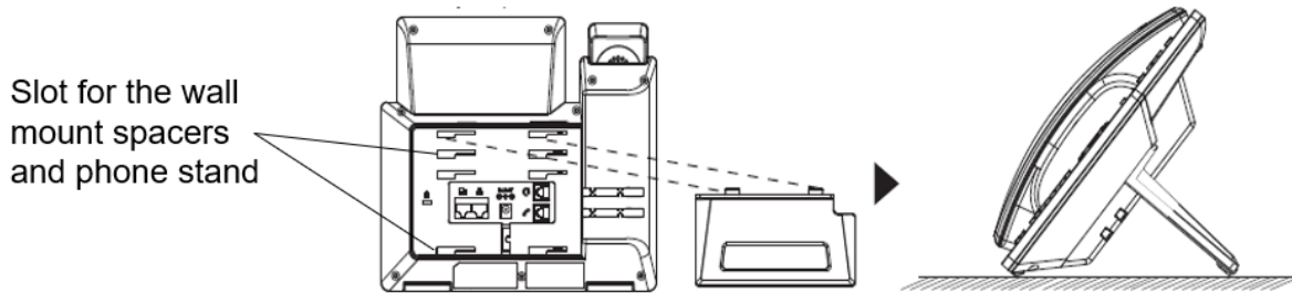
Figure 2: phone Stand and Mounting Slots on the GRP2600
